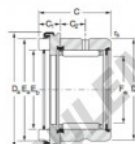
RAX 500 - RAXN 500
