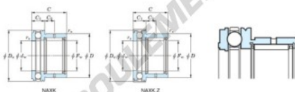
Boundary dimensions
