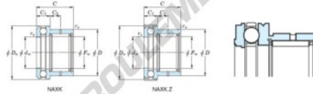
Ball thrust series
