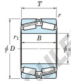
Boundary dimensions
