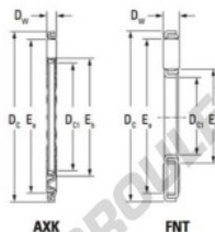
Boundary dimensions
