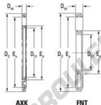
Boundary dimensions
