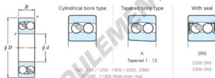
Boundary dimensions
