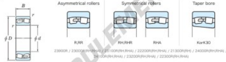
Spherical roller bearings
