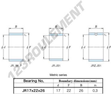
Boundary dimensions
